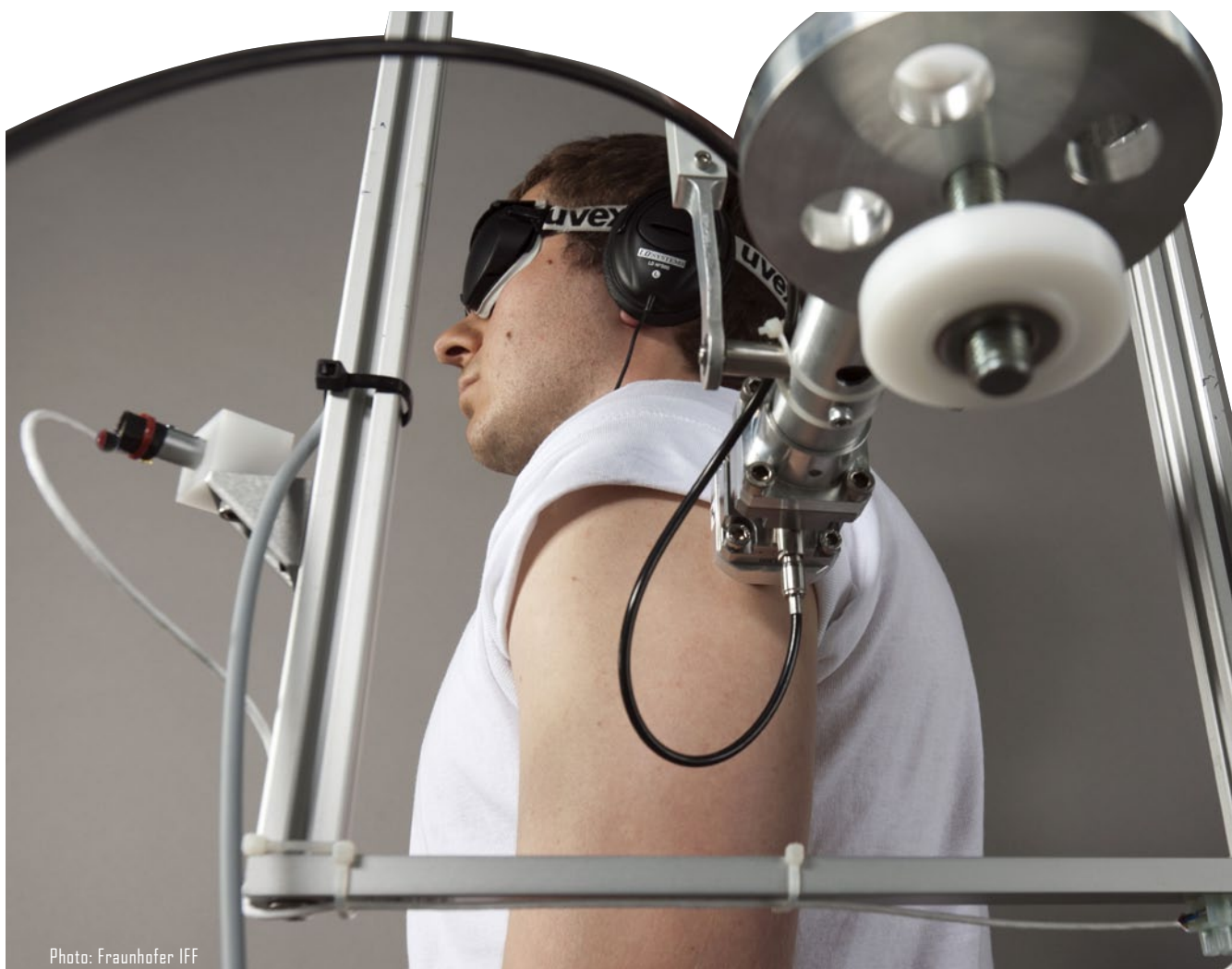
A subject during the study's impact test. How much force can act on a human body before a bruise appears?
